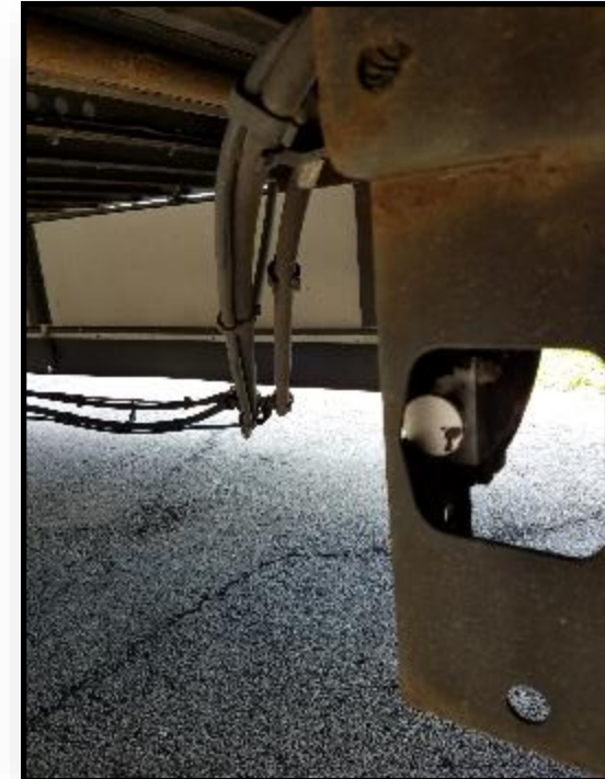
QUIK-DRAW® PNEUMATIC PIN-PULL MECHANISM
